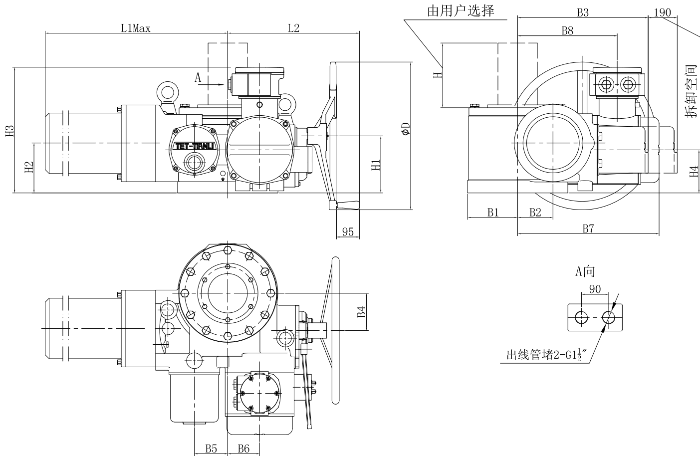
SMC-3~4整体型、防爆型、整体防爆型外形尺寸
